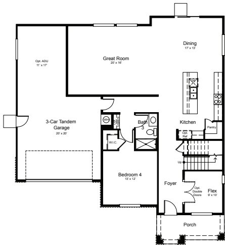
Floor 1 Elevation A - Tuscan
