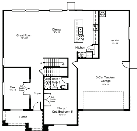
Floor 1 Elevation A - Tuscan
