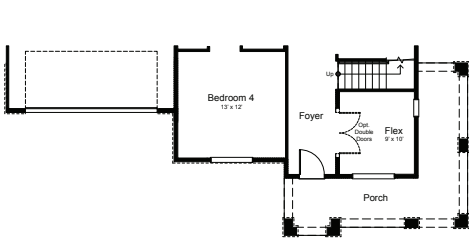
Opt. Wrap Around Porch at Elevation A
