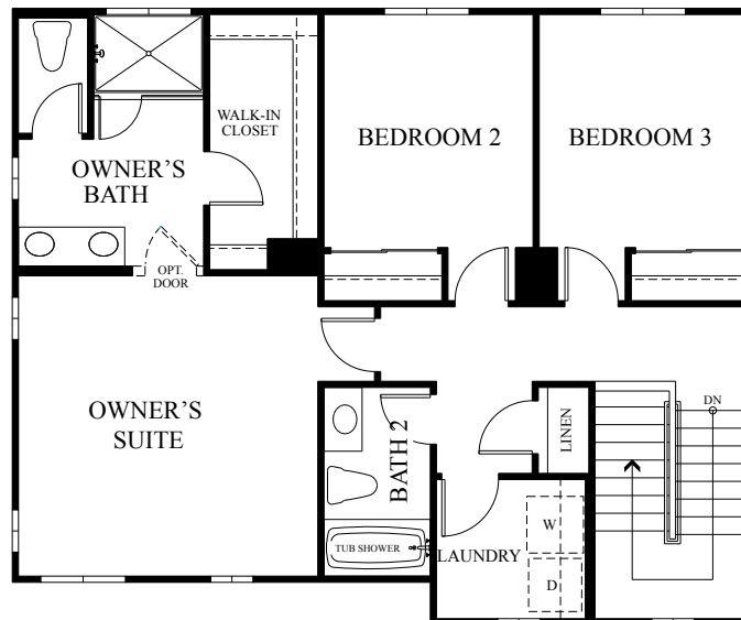
SECOND FLOOR
