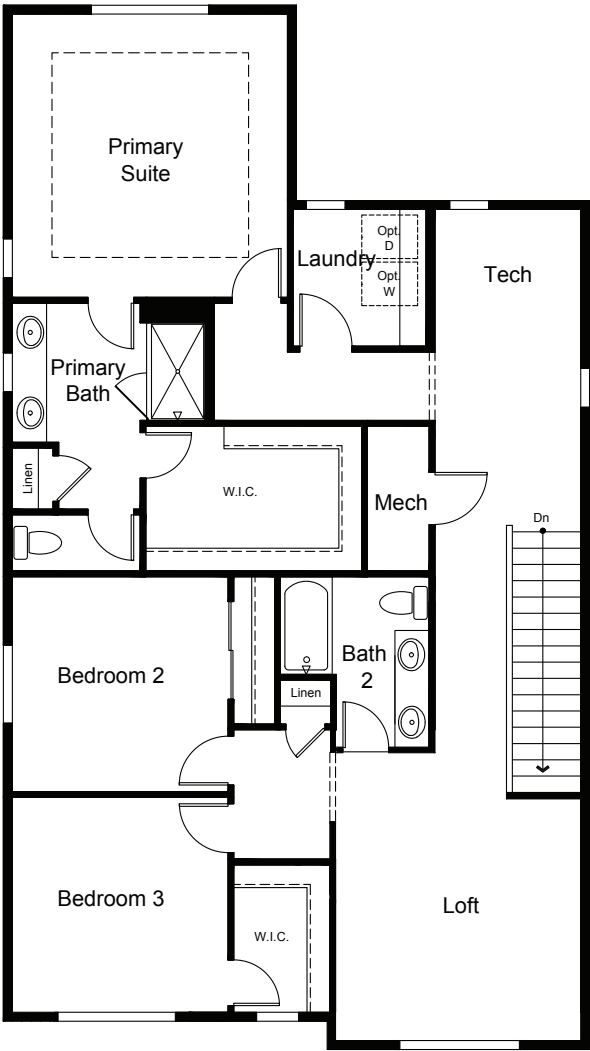
UPPER LEVEL
