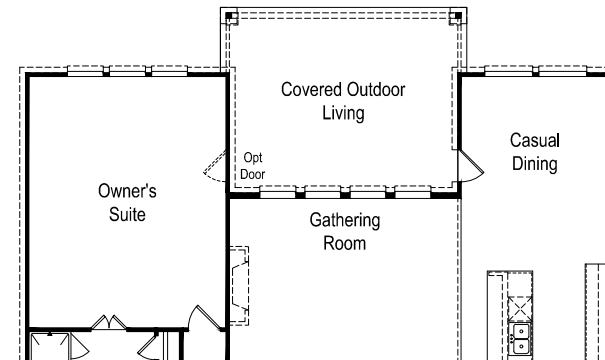
Opt Lifestyle Space - First Floor - Extends Game Room Above
